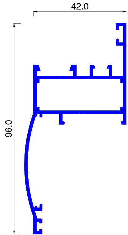
ALU435 kg/ml 0.902
