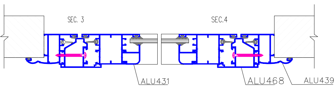
Section E-E
