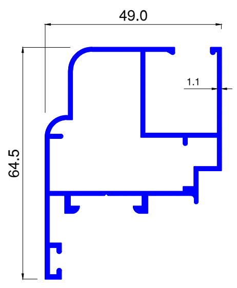
ALU480 kg/ml 0.815
