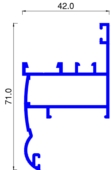
ALU439 kg/ml 0.799
