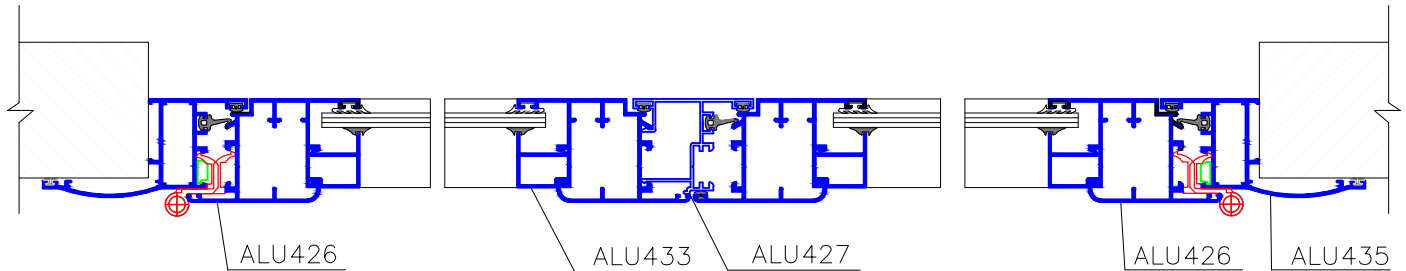
Section G-G
