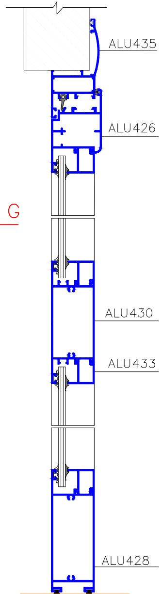
Section H-H
