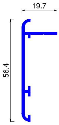
ALU450 kg/ml 0.338
