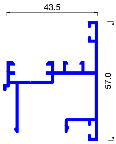
ALU427 Kg/ml 0.697
