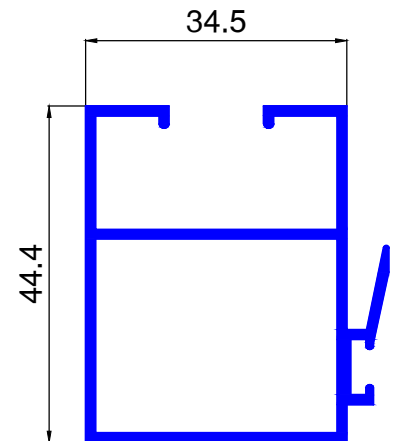
MT5372 0.689 kg/ml.
