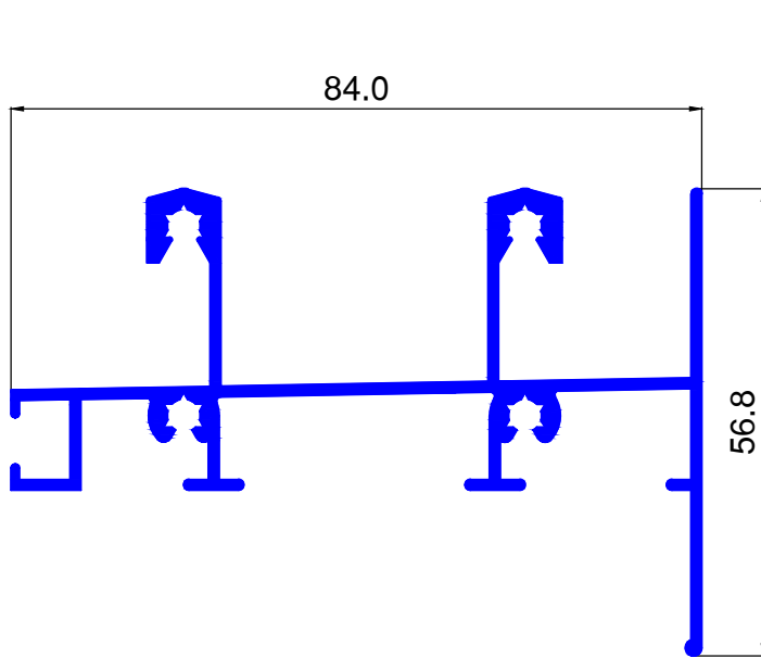
MT5370 1.180 kg/ml.
