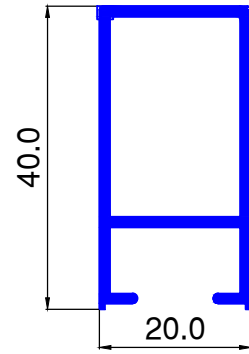
MT273 0.451 kg/ml.
