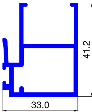
MT203 0.729 kg/ml.
