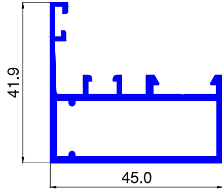
MT709 0.732 kg/ml.
