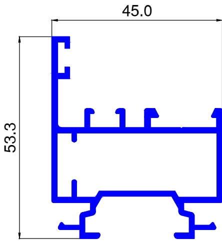
MT369 0.875 kg/ml.
