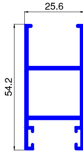
MT202 0.750kg/ml
