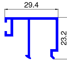
MT366 0.292 kg/ml.
