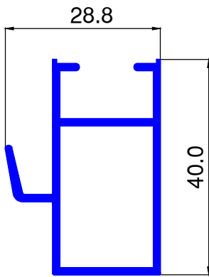
MT227 0.486 kg/ml.
