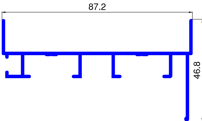
MT5371 0.759 kg/ml.
