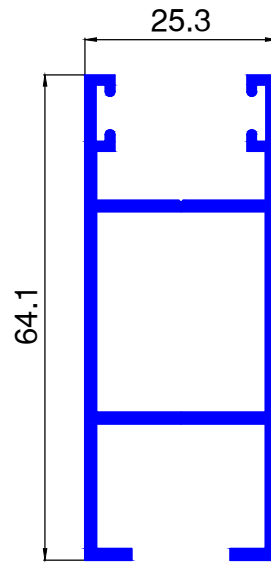
MT752 0.697 kg/ml.
