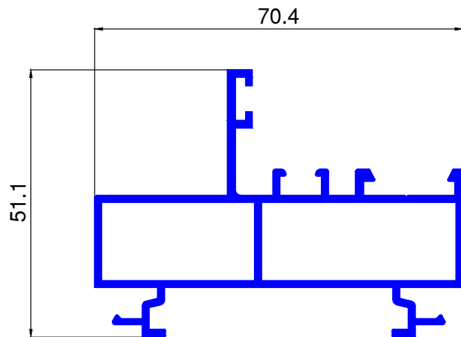
MT360 1.026 kg/ml.
