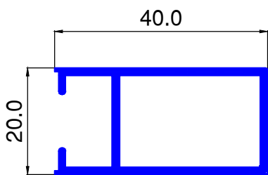
MT273 0.451 kg/ml.
