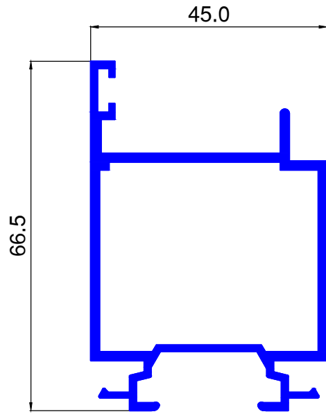
MT361 1.034 kg/ml.
