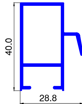
MT227 0.486 kg/ml.
