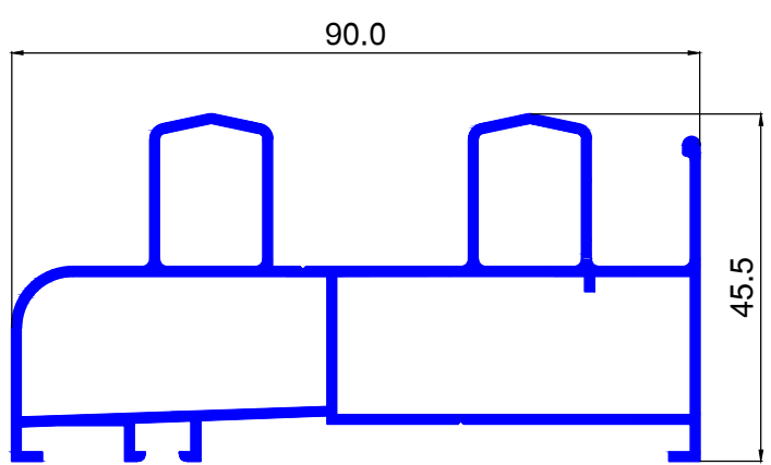
ALU646 Kg/ml. 1.239
