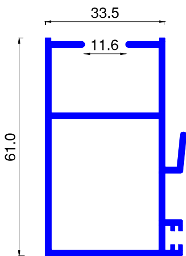
ALU623 Kg/ml. 0.980
