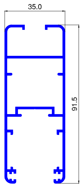
ALU634 Kg/ml. 1.118
