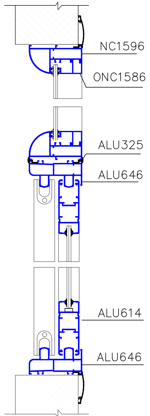
SEC. B-B
