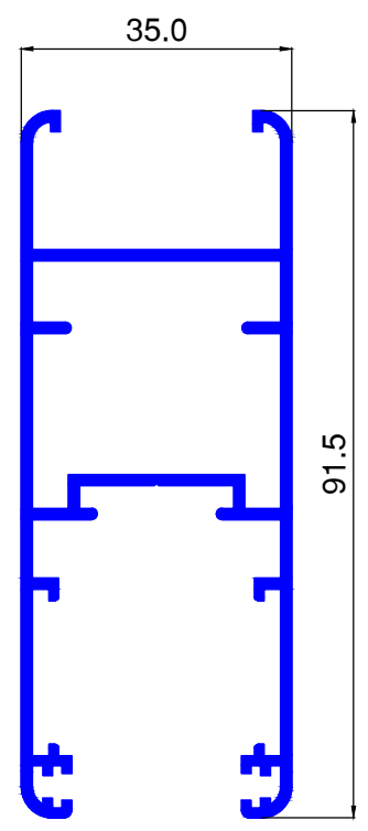
ALU635 Kg/ml. 1.177
