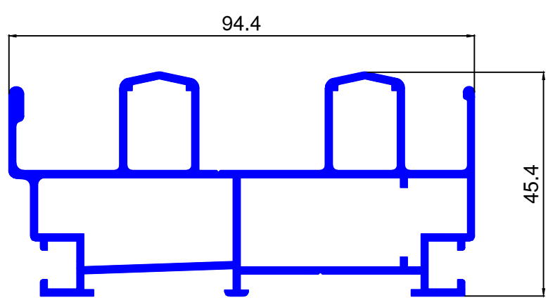
ALU646 Kg/ml. 1.239
