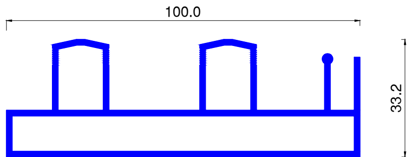
ALU626 Kg/ml. 1.501
