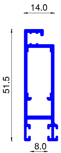
ALU320 Kg/ml. 0.554
