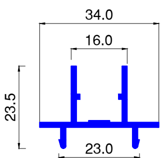
ALU318 Kg/ml. 0.332
