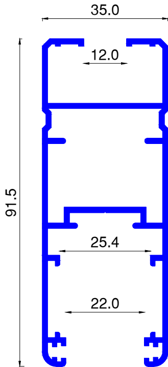
ALU614 Kg/ml. 1.239
