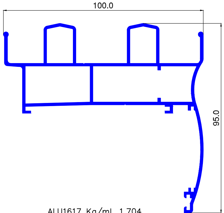
ALU1617 Kg/ml. 1.704
