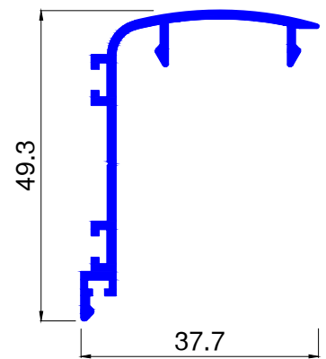
ALU630 Kg/ml. 0.394
