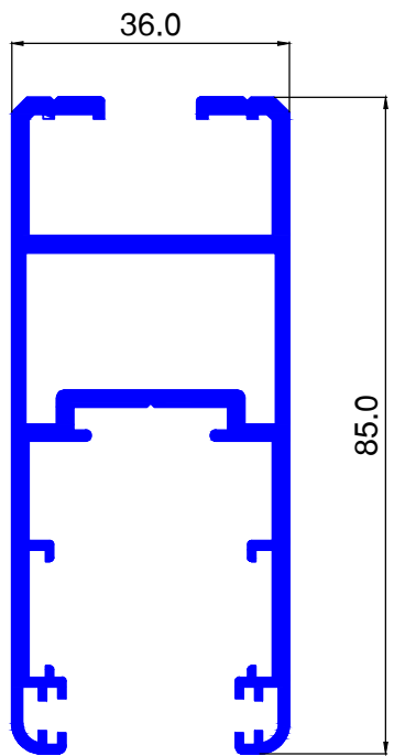
ALU606 Kg/ml. 1.609
